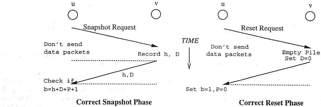
Fig. 7. Local snapshots and resets.
