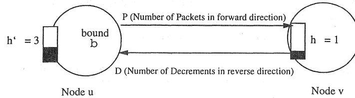
Fig. 5. Key variables for the bound estimation protocol on a link. The protocol maintains the invariant b = h + P + D + 1 .
