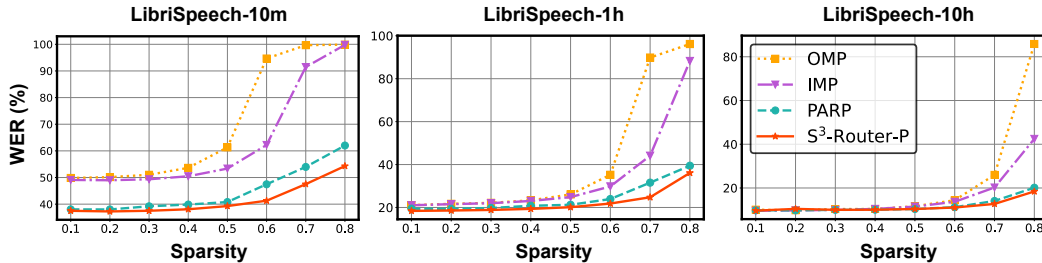
Figure 4: Benchmark our S^3 -Router-P against OMP, IMP, and PARP [93] for pruning wav2vec2-base on LibriSpeech. The WER on the test-clean set is reported.
