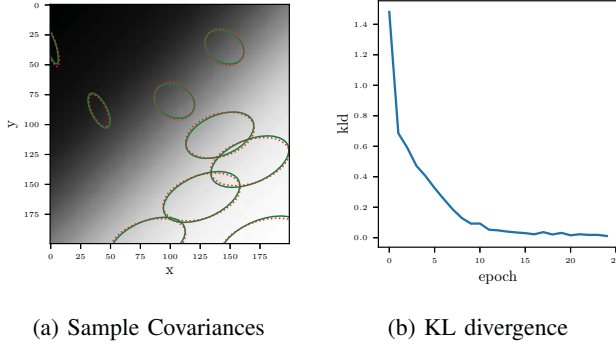
Fig. 3: Predicted covariance ellipses (red) and ground-truth covariance ellipses (green) are shown for a few samples in the simulated map. It can be seen that the Kullback-Leibler divergence is quickly reduced in just 25 epochs.
