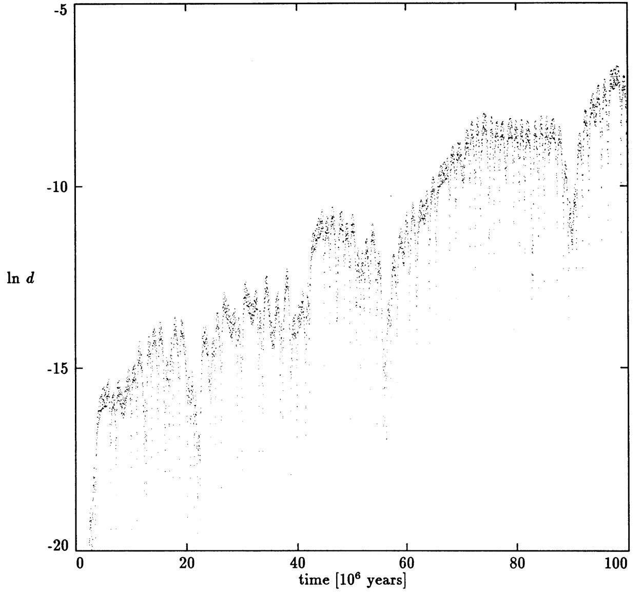
Figure 2: The divergence of the distance between the positions of Pluto in two different runs with very slight differences in initial conditions is characterized by a timescale near 12 million years.
