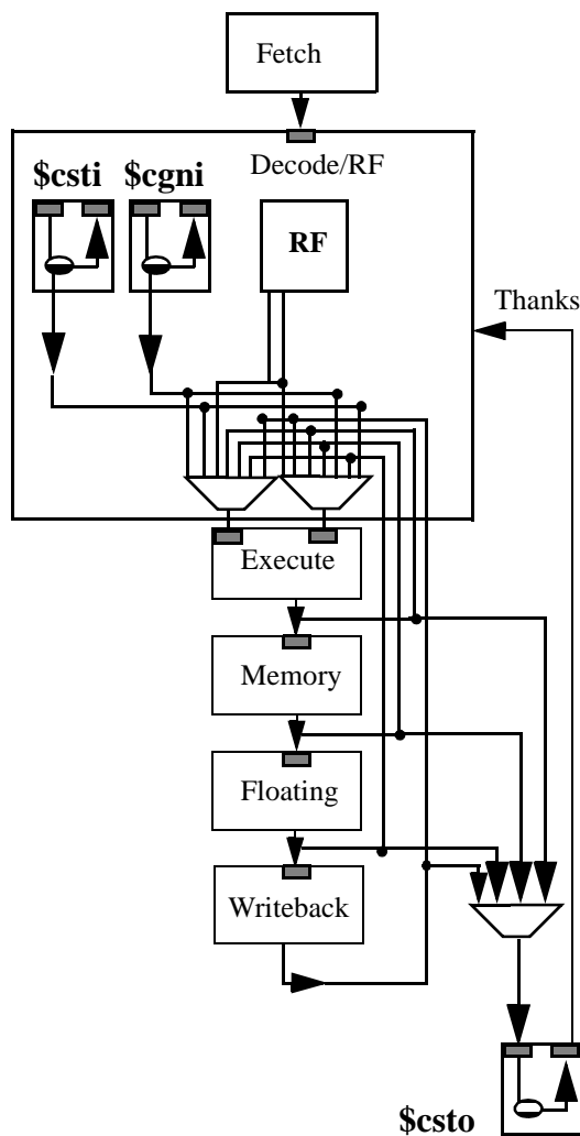
$csto, Bypass, and Writeback Networks
