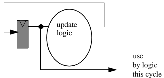
Circuitry for changes to all other SPRs
