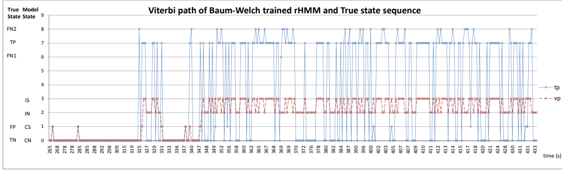
Figure 7-6: Viterbi path of an rHMM and the true state sequence. tp is the true state/event sequence, and vp is the inferred state sequence by the rHMM. In the dashed line, 0,1,2,3 in Y-axis correspond to the four states in Figure 7-4: clean and not suspicious (CN, corresponds to state 00), clean but suspicious (CS, to state 01), infected but not suspicious (IS, to state 10), and infected but suspicious (IS, to state 11). In the solid line, 0,1,6,7,8 represents an event that a host receives the following packets respectively: a normal packet (true negative, TN), an alert caused by false positives (FP), a clean signal caused by false negatives (false negative case 1, FN1), a true alert caused by an intrusion attempt (true positive, TP), a clean signal from a vulnerable host who cannot/would not distinguish intrusion attempts from normal traffic (false negative case 2, FN2).
