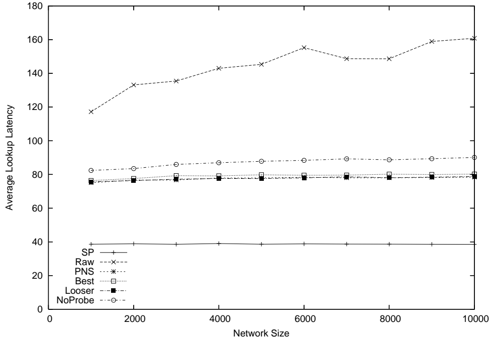
Figure 4-4: Synthetic topology: Average lookup latency.
