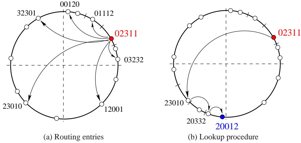
Figure 4-2: Pastry routing. In (a), the circle represents the name space, and the arrows show the entries in the routing table of node 02311, which is also shown in Table 4.1. (b) shows a lookup procedure by 02311 to find node 20012.
