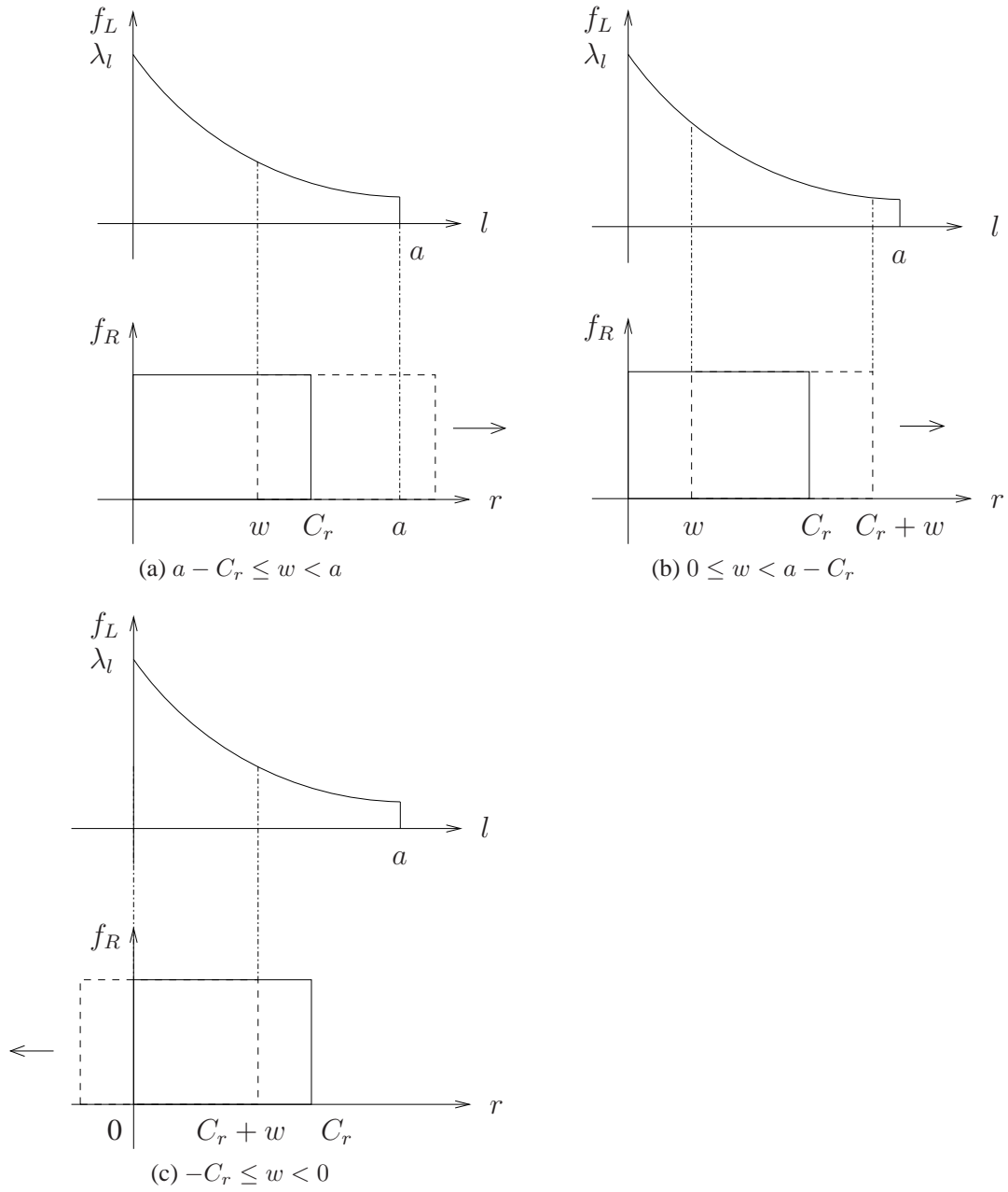
Figure A-2: Convolution in case B. The dashed rectangle shows the shift of f_R due to w .
