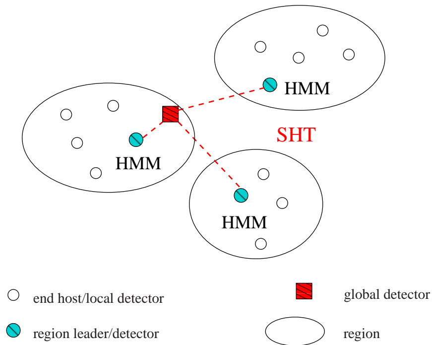
Figure 7-3: A region-based organization example.
