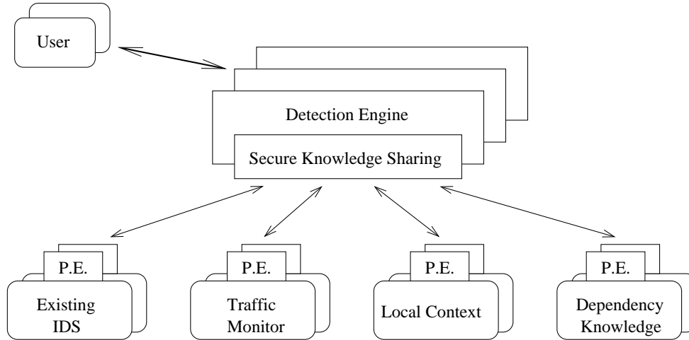
Figure 7-1: Knowledge-based intrusion detection framework. P.E. refers to “policy enforcer” described in Section 7.2.2.
