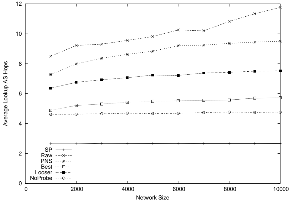
Figure 4-8: Real topology: Average lookup AS hops.
