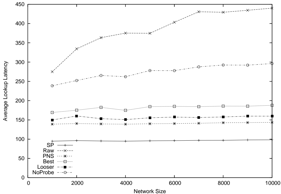
Figure 4-7: Real topology: Average lookup latency.
