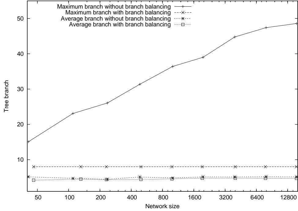
Figure 5-8: Tree branches against network size.
