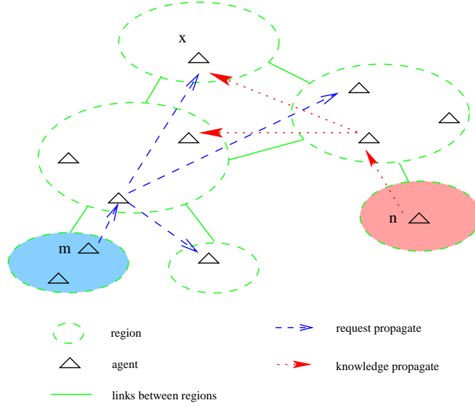
Figure 3-3: Request and knowledge propagation in the spec-KPs. This shows a request from agent m and a piece of knowledge from agent n meet at agent x .
