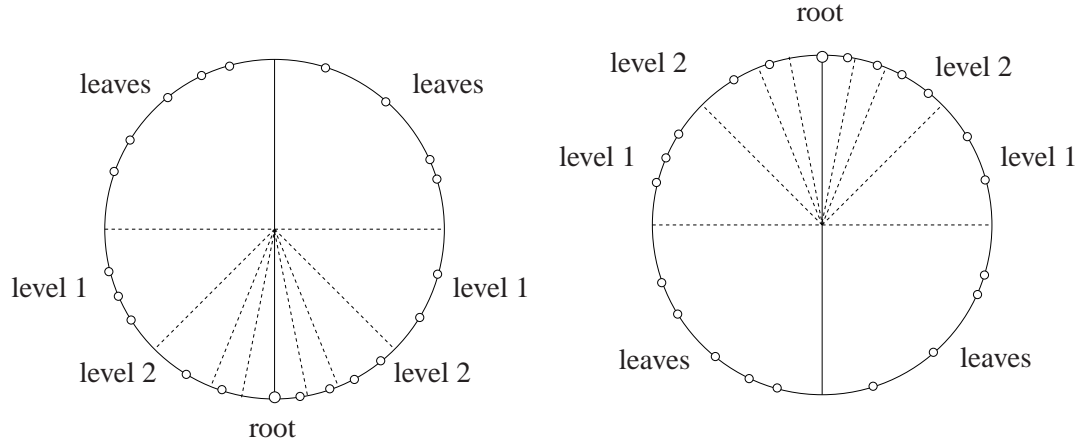
Figure 5-6: Two disjoint trees. Here k is 2, and the two roots are at 0 and \frac{m}{2} , respectively.
