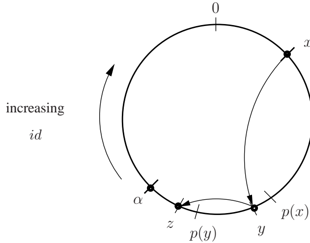
Figure 5-2: The node joining procedure. The circle represents the name space, \alpha is the root id , and the arrows show the directed edges of the tree from a child to its parent. In this figure, node y is node x 's parent in terms of P(x) . Node z is y 's parent in terms of P(y) .
