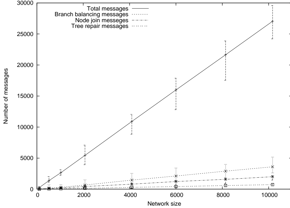
Figure 5-7: Communication overhead for tree construction.
