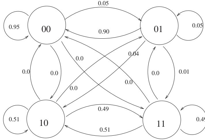
Figure 7-7: A trained hidden Markov model at a regional detector.
