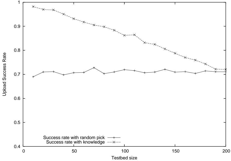
Figure 6-2: Upload success rate measurement.
