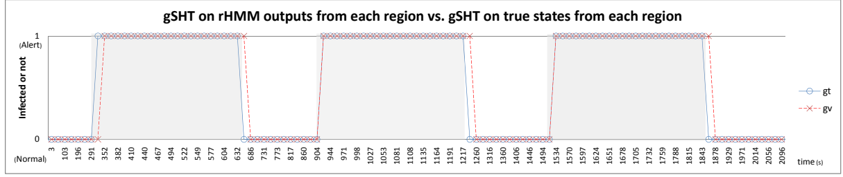
Figure 7-8: Global sequential hypothesis testing performance. gt is gSHT’s decision based on rHMM outputs, and gv is gSHT’s decision based on the true states from each region. Gray areas represent actual infection periods.
