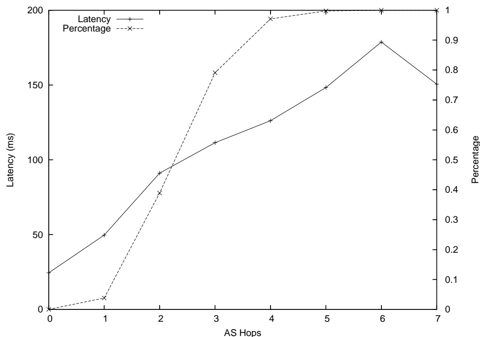
Figure 4-3: Relationship between AS hops and latency.
