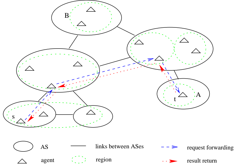
Figure 3-2: Request resolution in the NetKP. Agent s issues a request for the AS path between AS A and B . Agent s forwards the request to agents along the AS path, until it reaches agent t in AS A , as shown in the dashed arrow lines. Agent t checks its local knowledge base, and returns the corresponding AS path, as shown in the dotted arrow lines.
