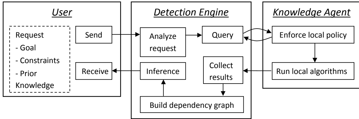
Figure 7-2: The resolution process of a request.
