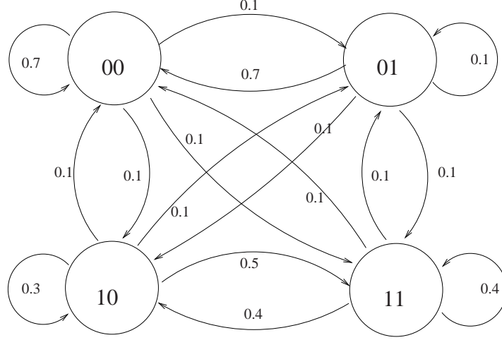
Figure 7-4: Initial Hidden Markov Model at regional detectors. 00 means the region is clean and its behavior is not suspicious, 01 means clean but suspicious, 10 means infected but not suspicious, 11 means infected and suspicious.
