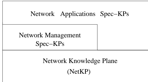
Figure 3-1: The system architecture. The underlying is the NetKP that provides application-independent network knowledge and facilities. On top of it, there are two parts: network management spec-KPs and network application spec-KPs. Network management spec-KPs is needed to support some network application spec-KPs.
