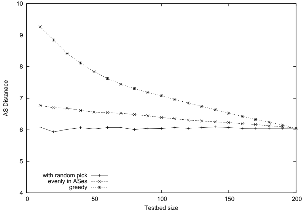
Figure 6-3: Node distribution experiment.
