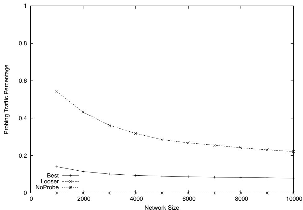
Figure 4-6: Synthetic topology: Probing traffic percentage.
