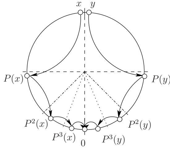
Figure 5-1: A tree example. The circle represents the name space, 0 is the root, and the arrows show the directed edges of the tree from a child to its parent. In this figure, node P(x) is node x 's parent, node P^2(x) is P(x) 's parent, and so on.
