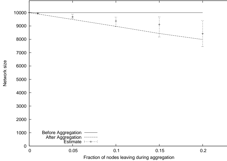
Figure 5-11: On demand estimation under various node failure rates.
