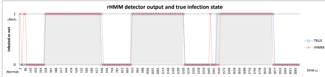
Figure 7-5: Regional Hidden Markov Model performance. TRUE is the states based on the true status (no false positive or false negative), and rHMM is that based on the observations of a regional detector. Gray areas represent actual infection periods.
