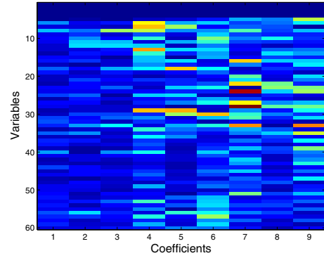
Figure 9: Coefficients associated to each of the k variables in the multinomial regularized model learned for algorithm MkRg3EDA.
