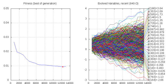
Figure 6: CMA-ES converging towards Nash VS number of function evaluations. The first graph on the left is the external fitness, while the graph on the right portrays the evolved genome
