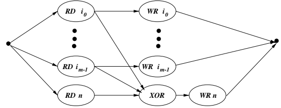
Figure 3: DAG3, Small Write DAG
