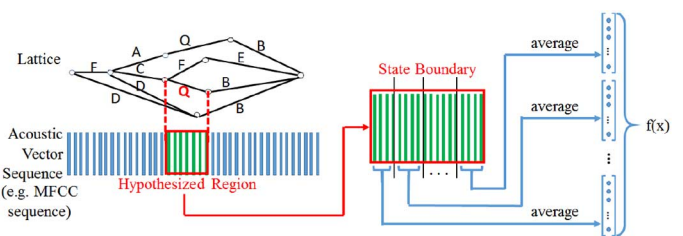
Fig. 5. Feature vector representations. Left half: a hypothesized region of the query term Q from the lattice. Right half: the feature vector f(x) .
