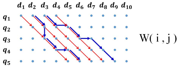
Fig. 8. The matching matrix W in (16) for D = (d_1, d_2, \dots, d_{10}) and Q = (q_1, q_2, \dots, q_5) with subsequence matching (red) or DTW (blue and thicker).
