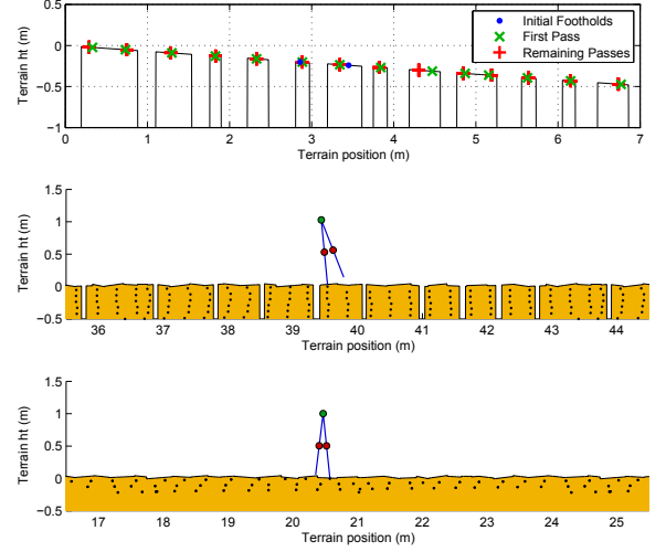
Fig. 19. Foothold patterns from optimal control. The optimal footholds on extreme terrain quickly converge to fixed pattern (top). On easier terrain, no fixed pattern emerges (bottom). In intermediate terrain, we see an intermediate level of organization in the pattern of footholds (middle). Footholds taken are plotted as dots in the lower two figures, with the earliest steps plotted lowest and with dots repeating as the terrain repeats, every 7 meters.
