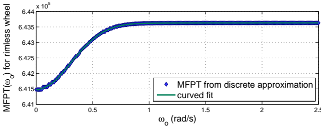
Fig. 6. Mean first-passage time as a function of the initial condition, \omega_o . Data are for a rimless wheel on stochastic terrain with mean slope of 8 deg and \sigma = 1.5^\circ . Points show the approximation obtained through eigen-analysis of the discretized system, and a smoothed line is overlaid. Note that MFPT is largely constant over a large portion of state space.
