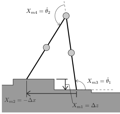
Fig. 28. Compass gait meshing parameters for stochastic terrain.
