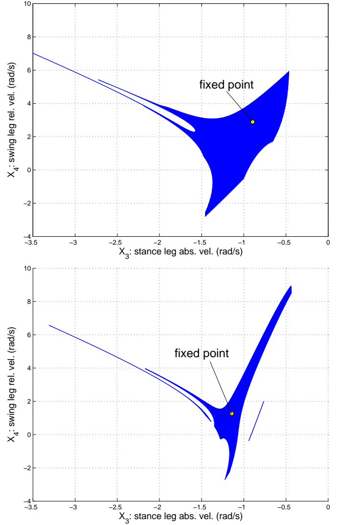
Fig. 12. Basins of attraction (blue regions) and fixed point for two compass walkers, each on a constant slope of 4^\circ . Walker with basin at top is more stable and uses the parameters defined for the stochastic system described throughout Section IV-B; for the other walker, m = m_h and a = b = .5 . MFPT is infinite inside the shaded region and is small (1-4 steps) outside of it. This image shows only a slice of the 3D basin, taken at the inter-leg angle of the fixed point for each respective walker. The fixed point is at X_3 = -.89 (rad/s), X_4 = 2.89 (rad/s), \alpha = 25.2^\circ for the first walker, and it is at X_3 = -1.14 (rad/s), X_4 = 1.26 (rad/s), \alpha = 33.4^\circ for the lower one. The deterministic basin of attraction for the second walker is narrower in shape, and this walker is significantly less stable on stochastic terrain.
