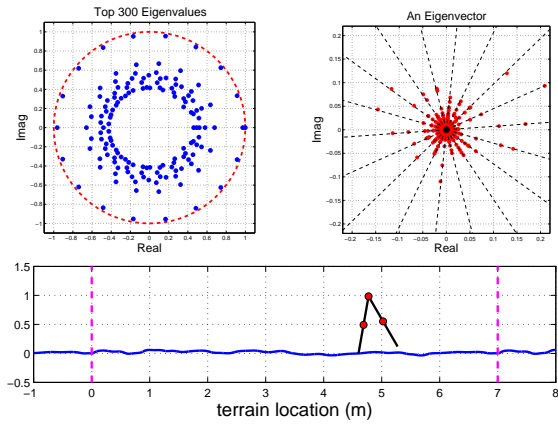
Fig. 24. Controlled compass gait walker, with torque at the hip. To solve for an optimal policy using value iteration, the terrain wraps every 7 meters. The optimization maximizes the MFPT from any given state. An eigen-analysis reveals a complex set of eigenvalues (top), spaced evenly about (but strictly inside of) the unit circle. Corresponding eigenvectors are also complex.
