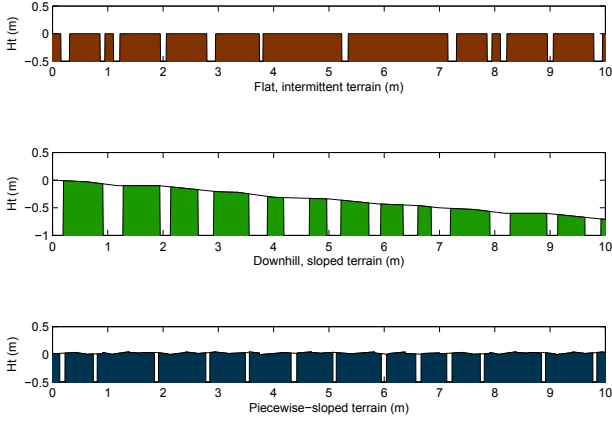
Fig. 17. Examples of terrain which were successfully negotiated using PD control alone. Without the added energy contribution of an impulsive toe-off, the actuated walker is limited to either mild variations in height or to terrain with an average gradient downhill. Terrain at top is flat except for a set of bottomless no-go gaps. The middle and bottom examples consist of piecewise slopes. Each was successfully solved both as a continuous terrain, shown as a solid black line, and as an intermittent terrain, represented by the solid regions. Figure 18 shows detail from the bottom plot.
