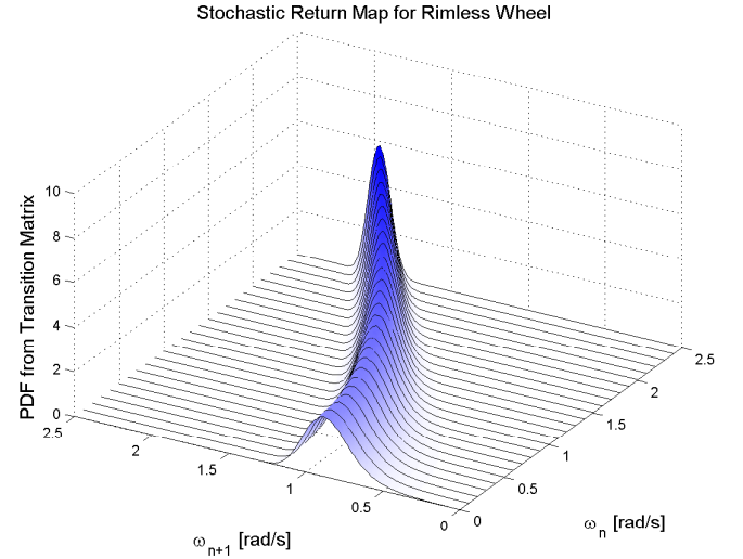
Fig. 5. 3D view of the return distribution for the stochastic rimless wheel system. This is a smoothed rendering of the step-to-step transition matrix, T , with the probability density functions for some particular values of \omega_n overlaid as lines for greater clarity.
