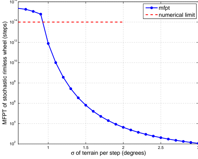
Fig. 9. Mean first-passage time (MFPT) for the rimless wheel, as a function of terrain variation, \sigma . Estimates above 10^{14} correspond to eigenvalues on the order of 1 - 10^{-14} and are beyond the calculation capabilities of MATLAB.
