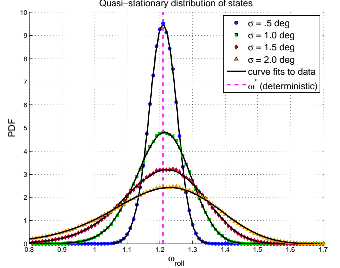
Fig. 7. Quasi-stationary probability density functions for the stochastic rimless wheel for each of several values of terrain noise, \sigma . Each distribution is estimated by renormalizing the eigenvector associated with the second-largest eigenvalue of the transpose of the transition matrix. Note that meshing inherently adds noise to the dynamic system; smoothed lines are drawn on top of the raw data (shown as points) from the scaled eigenvectors.
