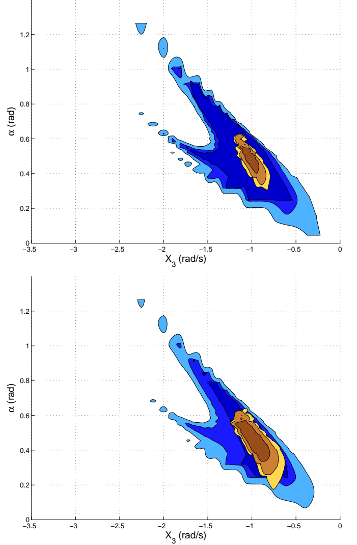
Fig. 14. Metastable system: Contours of the stochastic “basin of attraction” are shown where MFPT is 0.5M , 0.9M and 0.99M (blue) versus contours where the integral of the PDF accounts for .9, .99, and .999 of the total metastable distribution (yellow). The metastable dynamics tend to keep the system well inside the “yellow” neighborhood. As the tails of this region extend out of the blue region, the system dynamics become less stochastically stable (lower M ). The axis into the page represents the swing leg relative velocity, X_4 , and a slice is taken at X_4 = 2.33 (rad/s). Terrain variability for the top plot is \sigma = 0.5 degrees (with M \approx 180,000 steps). For the noisier system at bottom ( \sigma = 1.0 degrees), M is only 20 steps or so.
