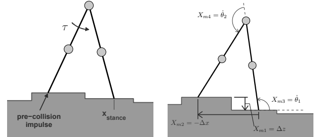
Fig. 21. Compass gait on stochastic terrain. At left, the actuation for this model again includes a torque at the hip and a constant magnitude impulse which occurs at each step. At right, the four states which define each post-collision elements in the discrete mesh are given.
