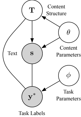
Figure 2: A graphical depiction of the generative process for a labeled document at training time (See Section 3); shaded nodes indicate variables which are observed at training time. First the latent underlying content structure \mathbf{T} is drawn. Then, the document text s is drawn conditioned on the content structure utilizing content parameters \theta . Finally, the observed task labels for the document are modeled given s and \mathbf{T} using the task parameters \phi . Note that the arrows for the task labels are undirected since they are modeled discriminatively.
