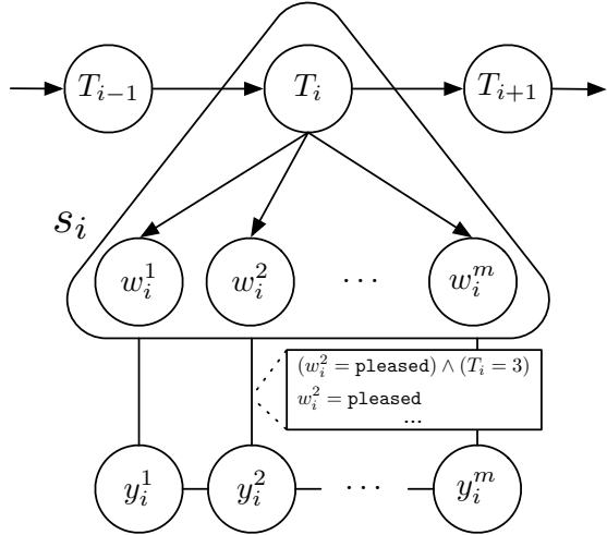
Figure 1: A graphical depiction of our model for sequence labeling tasks. The T_i variable represents the content model topic for the i th sentence s_i . The words of s_i , (w_i^1, \dots, w_i^m) , each have a task label (y_i^1, \dots, y_i^m) . Note that each token label has an undirected edge to a factor containing the words of the current sentence, s_i as well as the topic of the current sentence T_i .
