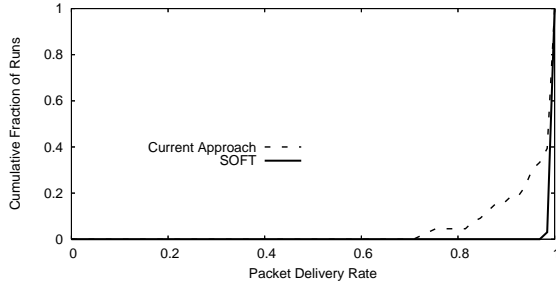
Figure 9: CDFs of Delivery Rates in Low Loss Environments. We use the same power as before but with DSSS, which improves the delivery rates for both SOFT and the current approach. For these environments, SOFT eliminates all losses for the vast majority of the runs.
