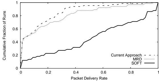
Figure 5: CDF of Packet Delivery Rates. SOFT significantly improves the packet delivery rate in lossy and low-coverage networks. While the mean delivery rate in the current approach and MRD is less than 7%, the mean SOFT delivery rate is as high as 62%. Retransmissions are turned off in these experiments, thus the improvement in delivery rate is mainly due to the use of soft values and the effect of spatial diversity.
