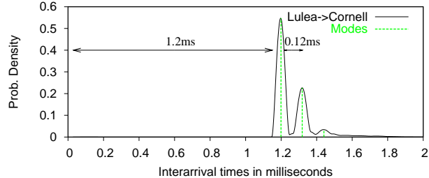
(b) Upstream highly congested 100 Mb/s and downstream 10 Mb/s.
