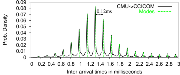
(b) Gaps of 0.12ms show the 100Mb/s CCICOM link
