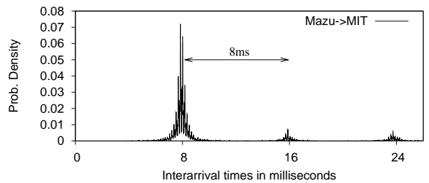
(a) Upstream congested T1 and downstream 100 Mb/s.
