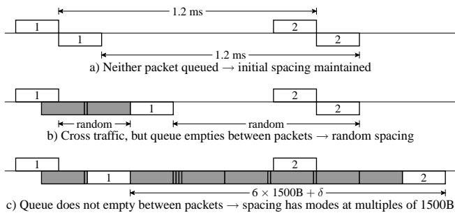
Figure 3—Various cases of packet spacing on CCICOM's access link. Arrivals are shown above the line, departures below the line. Light packets are from the traced flow and dark packets are cross traffic. Cross traffic arrivals are not shown.
