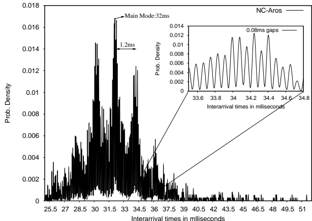
(c) Three bottlenecks. The envelope peaks at 32 ms, indicating an upstream 380 Kb/s link; 1.2 ms EMGs correspond to the 10 Mb/s downstream link; and 0.08 ms EMGs in the zoomed figure show a 155 Mb/s bottleneck.
