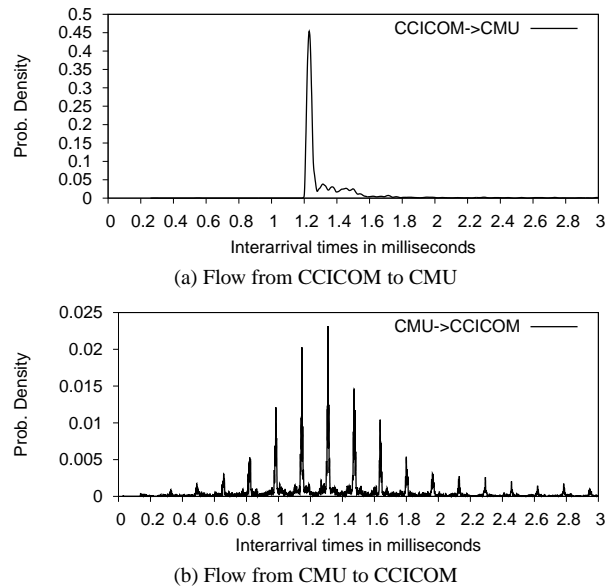
Figure 2—Interarrival PDFs for CCICOM–CMU path in both directions.
