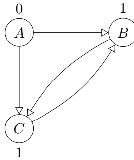
Figure 7.6: A predecessor graph, (A, B) and (A, C) are mutually dominant.
