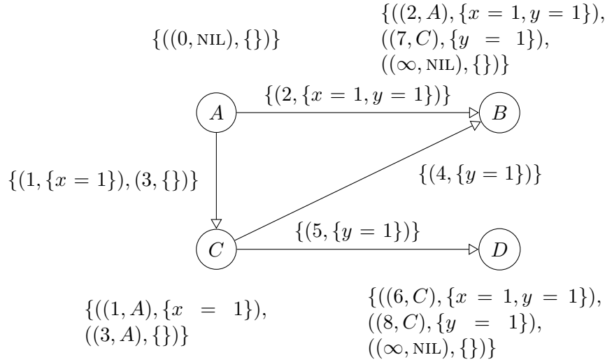
(a) Relaxed Graph
