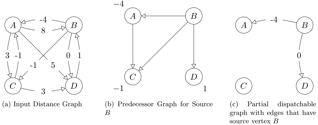
Figure 7.2: A single step of the fast reformulation algorithm for STNs
