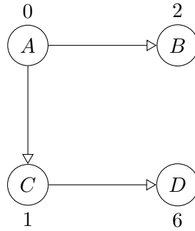
(b) Predecessor graph for e = \{x = 1, y = 1\}
