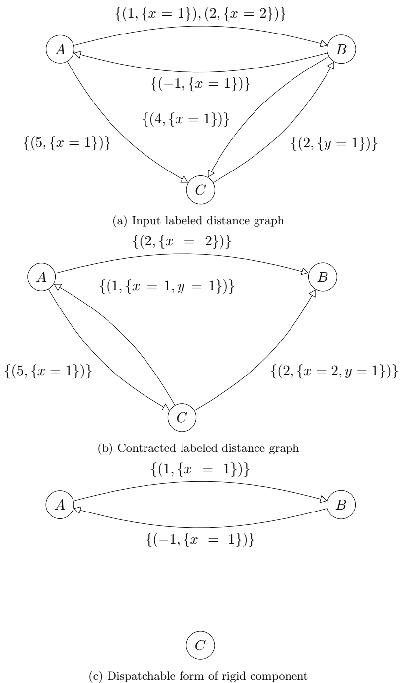
Figure 7.8: An example of processing a rigid component from a Labeled Distance Graph.
