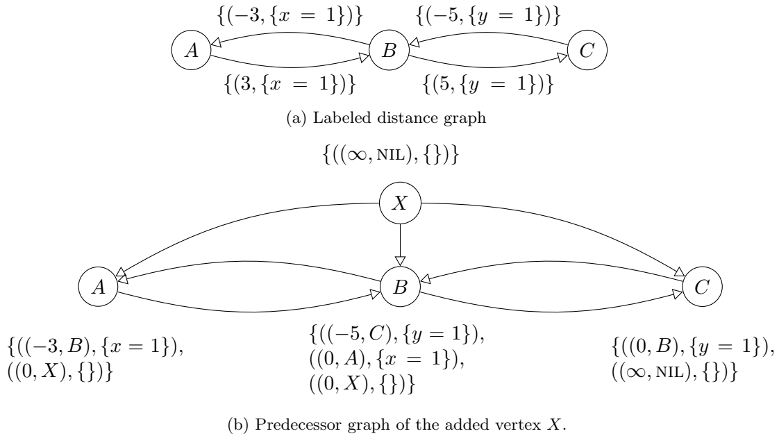
Figure 7.7: Identifying rigid components in labeled distance graphs.
