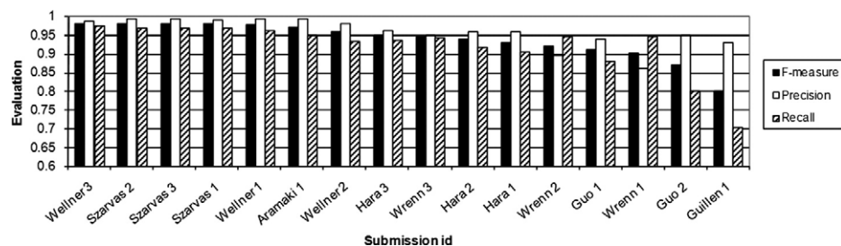
Figure 2. System Comparison Based on Overall Token-Level Performance on PHI (rank ordered in F-measure).
