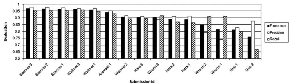
Figure 8. System Comparison Based on Overall Instance-Level Performance on PHI (rank ordered by F-measure). Guillen's output did not meet our instance-level evaluation requirements and was therefore excluded from this evaluation.
