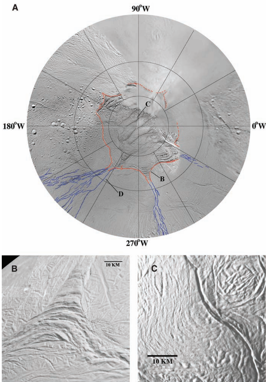
Fig. 2. (A) Polar stereographic basemap of the SPT covering latitudes from 0° to 90°S. The basemap also shows details obtained from the best ISS coverage of Enceladus' SPT to date. The circumpolar tectonic margin that encloses the SPT is marked as solid red lines where it is well resolved in high-resolution ISS images and as dashed red lines where it is interpreted from low-resolution coverage. Blue lines identify prominent, young tension fractures that extend from the Y-shaped discontinuities north to the equator. (B) Morphological details of a Y-shaped discontinuity along the SPT margin near 44°S, 279°W. North is up and the image scale is 70 m/pixel. (C) Example of grooved bands in bright plains adjacent to a tiger stripe at 86°S, 102°W. Note how the bands curve to define a quasi-circular feature. (D) Transition of Y-shaped discontinuity at the polar terrain boundary near 30°S, 229°W to north-south-trending fractures extending to the equator (blue lines in Fig. 3A).
