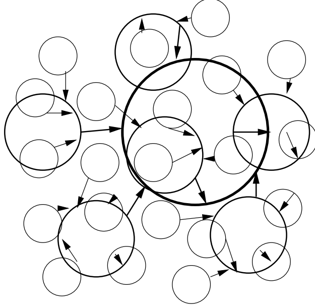
Figure 3: A hierarchy of three levels of nodes. Larger circles are higher-level nodes, and arrows show parentage relations between a nodes.
