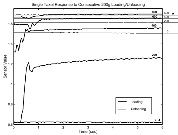
Figure 4.8: Response of a single taxel to consecutive 200-gram loads followed by their consecutive removal. Note the hysteresis.
