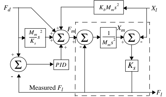
Figure 8: Control Architecture
