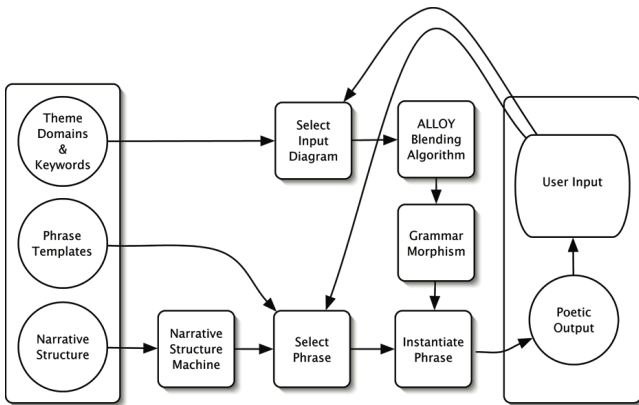
Figure 1: The GRIOT System Architecture
