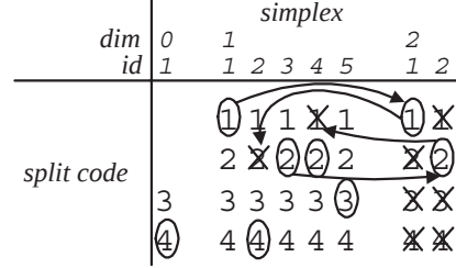
Figure 6: Constraints on the split codes for the simplices in the example of Figure 5.
