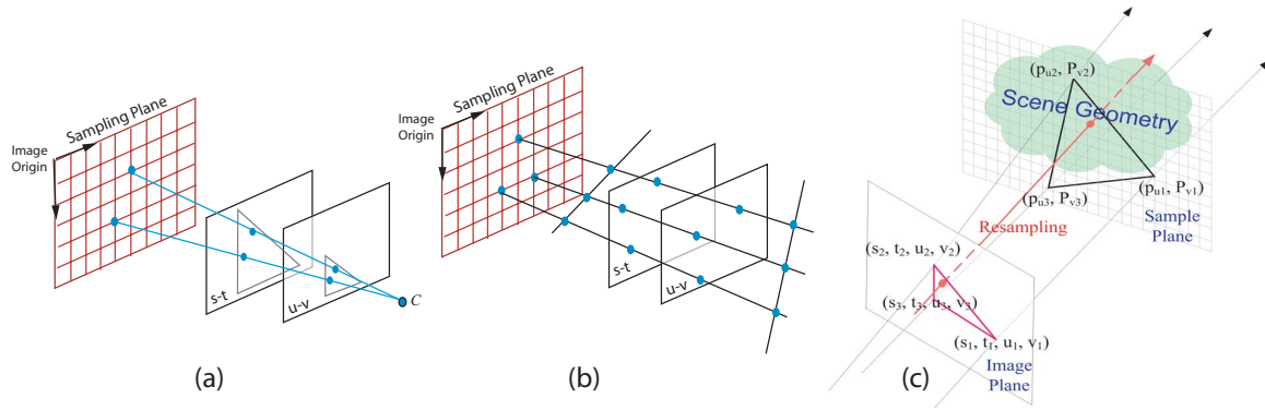
Figure 7: (a) Sampling of a pinhole camera (homography). (b) Sampling of a cross-slit camera. (c) Sampling of an arbitrary multiperspective image is achieved by assigning a sampling plane to each GLC.
