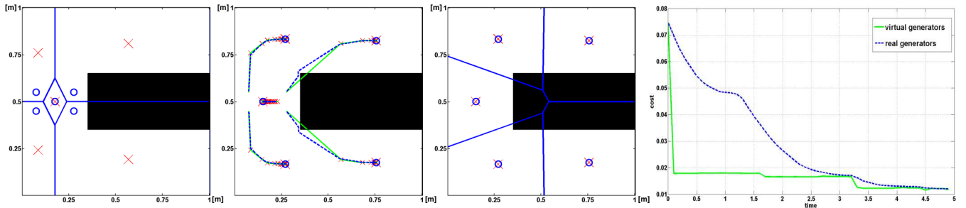
Fig. 3. Voronoi coverage in a U-shaped environment (obstacle in black). From left to right: five robots (blue circles) start from an initial position and move along the shown trajectories from one current target to the next target (red crosses) until they reach a final configuration. The next target is computed by the Lloyd algorithm as soon as a robot reaches its current target. The green lines illustrate the trajectories of the virtual generators. Two green lines intersect the obstacle’s corners and show that an obstacle avoidance behavior is needed to cover this environment. The cost \mathcal{H} for the configuration of the virtual and the real generators over time is shown in the plot on the right.
