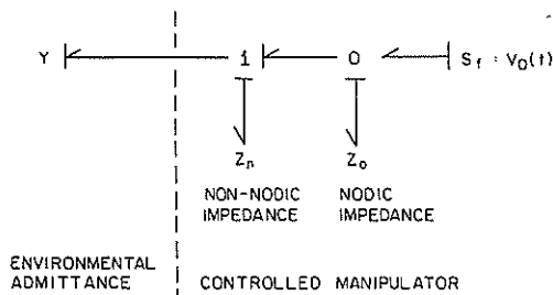
Fig. 5 A bond graph equivalent network representation of the minimum necessary structure of an impedance-controlled machine including both nodic ( Z_0 ) and non-nodic ( Z_n ) impedance
