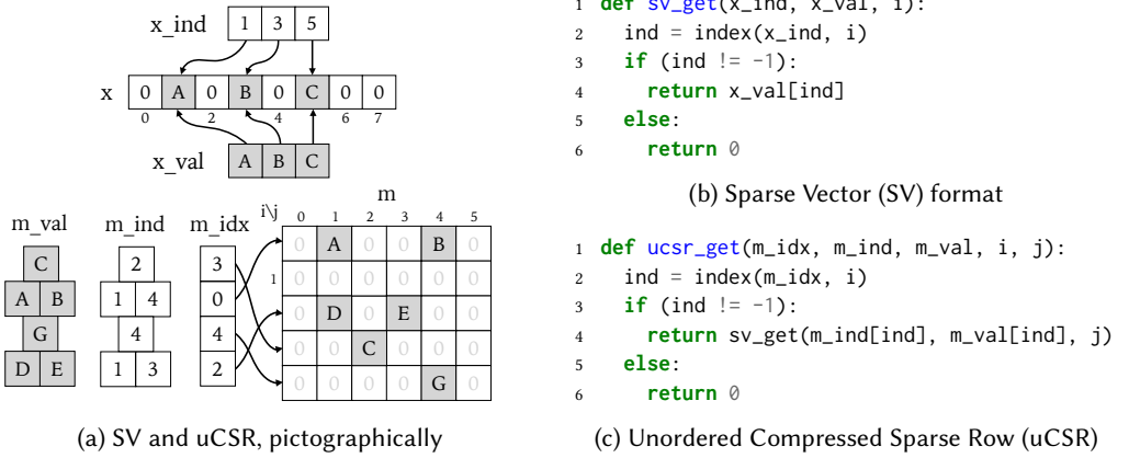
Fig. 2. Sparse Vector and Unordered Compressed Sparse Row formats
