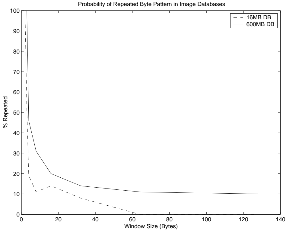
Figure 3-5: Probability of Repeated Byte Patterns in Image Databases
