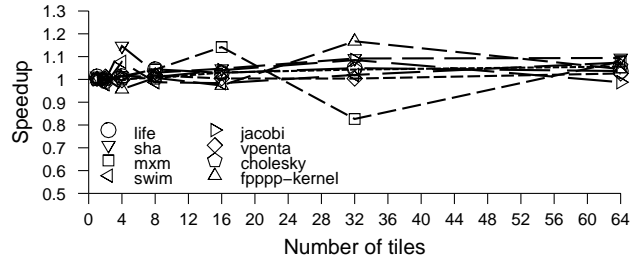
Figure 14: Impact of removing contention.
