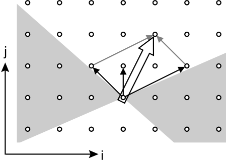
Figure 5: Iteration space diagram for Example 1. Here the hollow arrow denotes an Affine Occupancy Vector that is valid for all legal affine schedules. The gray region indicates the slopes at which a legal affine schedule can sweep across the iteration domain.
